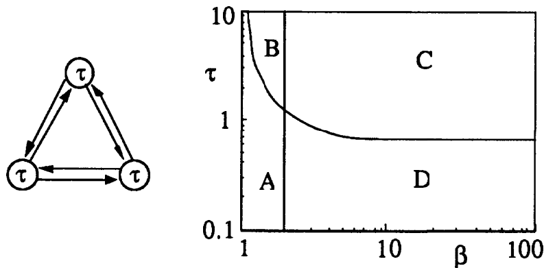
Figure 2. Stability Diagram for the All-Inhibitory Delay Network for the Case N = 3 . See Text for a Description of A,B,C and D.
