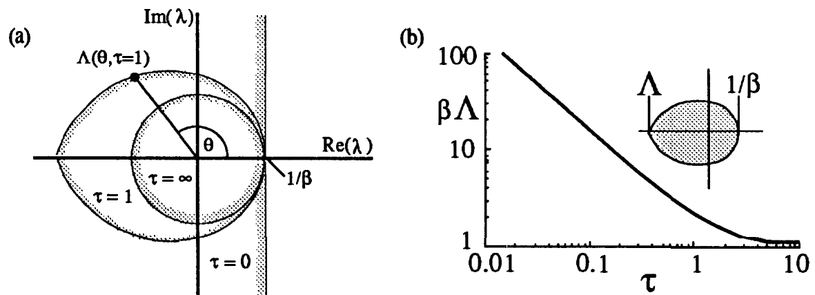
Figure 1. (a) Regions of Stability in the Complex Plane of Eigenvalues \lambda of the Connection Matrix J_{ij} for \tau = 0, 1, \infty . (b) Where Stability Region Crosses the Real- \lambda Axis in the Negative Half Plane.
