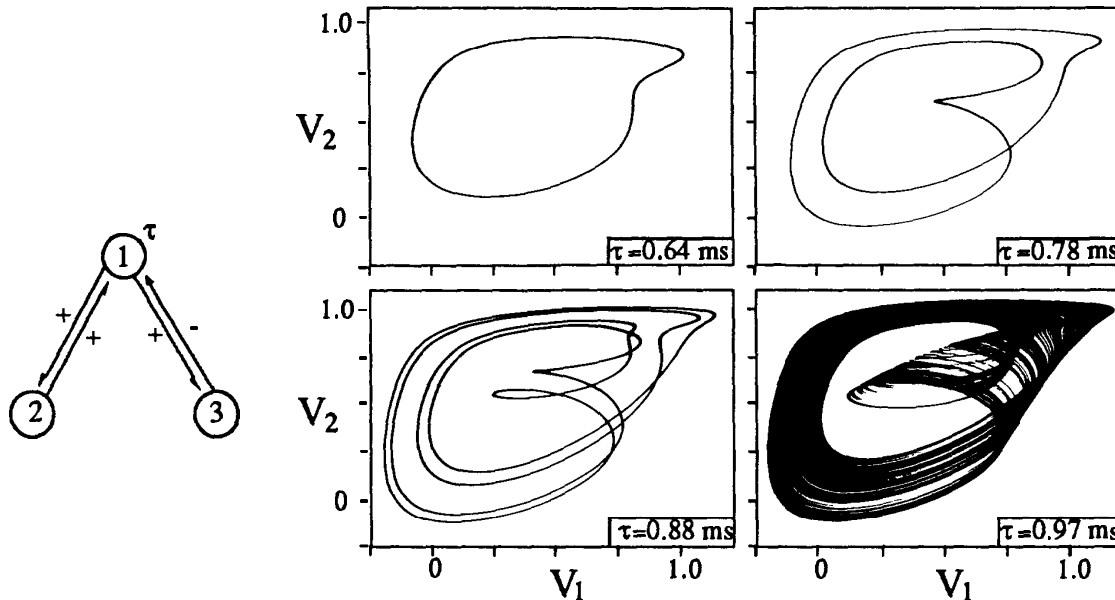
Figure 4. Period Doubling to Chaos as the Delay in Neuron 1 is Increased.
