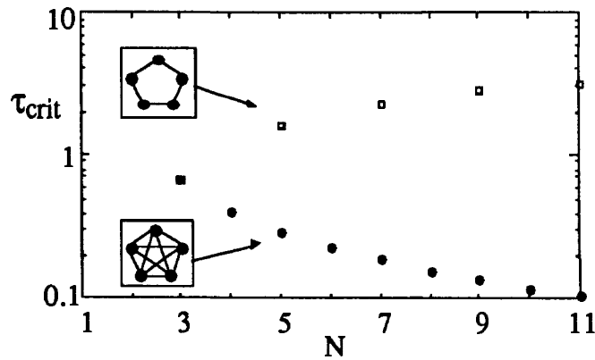
Figure 3. Critical Delay from Large-Gain Theory for All-Inhibitory Networks (circles) and Frustrated Rings (squares) of size N .
