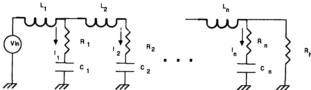
Figure 4 - Transmission line model of the cochlea represented as an electrical circuit.
