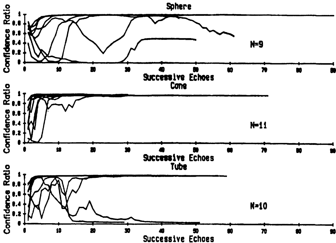
Figure 2. Results of generalization testing of the network in the form of the confidence of the network in assigning the echo train to the proper category. See text.
