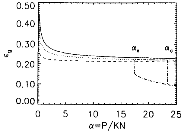
Figure 3: Generalization error for continuous weights and T = 0.5 . The approach to the residual error is shown including 1/\sqrt{K} -corrections for K=5 (solid line), K=11 (dotted line), and K=100 (dashed line). The broken line corresponds to the solution with nonvanishing \Delta .
