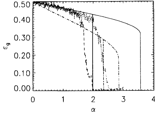
Figure 1: Learning curve for the large- K tree committee (solid line) with binary weights at T = 1 . The phase transition occurs at \alpha_c = 1.98 , and the spinodal point is at \alpha_s = 3.56 . The analytic results are compared with Monte Carlo simulations with K = 9 , N = 75 and T = 1 , averaged over 10 runs. In each simulation the number of training examples is gradually increased (dotted line) and decreased (dashed line), respectively. The broken line shows the generalization error for the simple perceptron.
