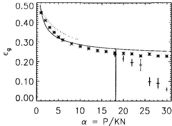
Figure 4: Generalization error for binary weights at T = 5 . The large- K theory for different regions of \alpha is compared with simulations for K = 5 and N = 45 averaged over all simulations (+) and simulations, in which no freezing occurred (*), respectively. The solid line shows the finite- \alpha results including 1/\sqrt{K} -corrections. The dotted line shows the small- \alpha solution.
