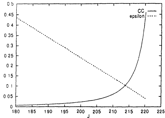
FIGURE 1. The equal-time cross-correlations between a pair of excitatory neurons, and the real part of its inverse time-constant, \epsilon , vs. the excitatory coupling parameter J .
