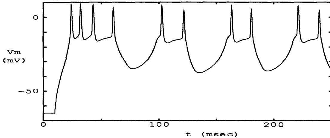
Figure 3: Dendritic calcium spikes. All-or-nothing dendritic Ca^{2+} calcium spikes can be generated by adding a voltage-independent but Ca^{2+} -dependent K^+ conductance to the apical tree with g_{max} = 11.4 \text{ nS} . The trace shown is in response to sustained intradendritic current injection of 0.5 \text{ nA} . For clamp currents of 0.3 \text{ nA} or less, no calcium spikes are triggered and only single somatic spikes are obtained (not shown). These currents do not substantially affect the current amplifier effect.
