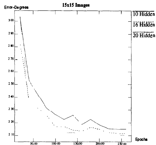
Figure 3: Error vs. Epochs for the 15x15 images. Errors shown for the 2000 image test set. Each line represents three ANN trainings per user; two users are tested.
