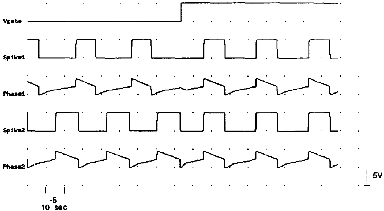
Figure 4: Phase-Locking Simulation
