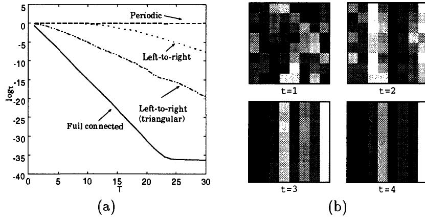
Figure 2: (a) Convergence of Dobrushin's coefficient (see Definition 3). (b) Evolution of products A^{(1,t)} for fully connected graph. Matrix elements are visualized with gray levels.
