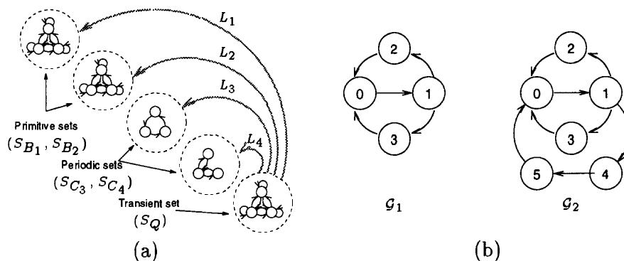
Figure 1: (a): Transition graph corresponding to the canonical decomposition. (b): Periodic graph \mathcal{G}_1 becomes primitive (period 1) \mathcal{G}_2 when adding loop with states 4,5.
