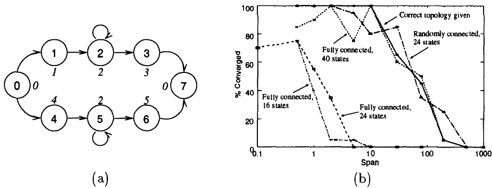
Figure 3: (a): Generating HMM. Numbers out of state circles denote output symbols. (b): Percentage of convergence to a good solution (over 20 trials) for various series of experiments as the span of dependencies is increased.
