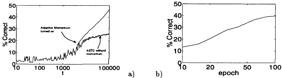
Figure 4: Phoneme Classification: Percent Correct a) ASTC without momentum (bottom curve) and adaptive momentum (top) as function of the number of input presentations. b) Conjugate Gradient Descent – one epoch equals one pass through the data, i.e. 9000 input presentations.
