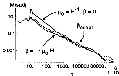
Figure 2: 4-D LMS with \rho = 10^5 : Plot displays misadjustment. Annealing starts at t = 10 . For \beta_{adapt} and \beta = I - \mu_0 \mathcal{H} , we use \mu_0 = .5 . Each curve is an average of 10 runs.
