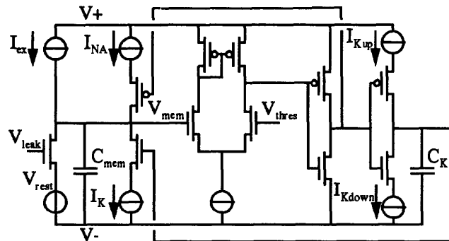
Fig. 3. The Spiking Neuron circuit
