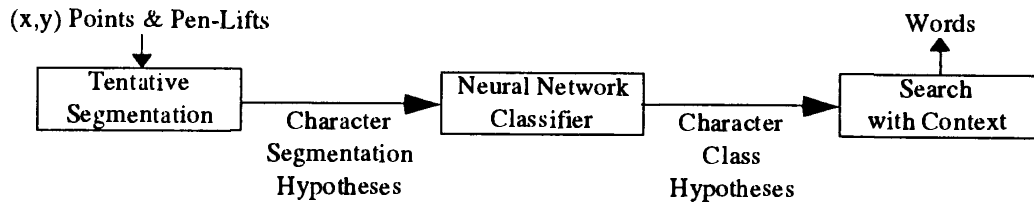
Figure 1: A Simplified Block Diagram of Our Hand-Print Recognizer.
