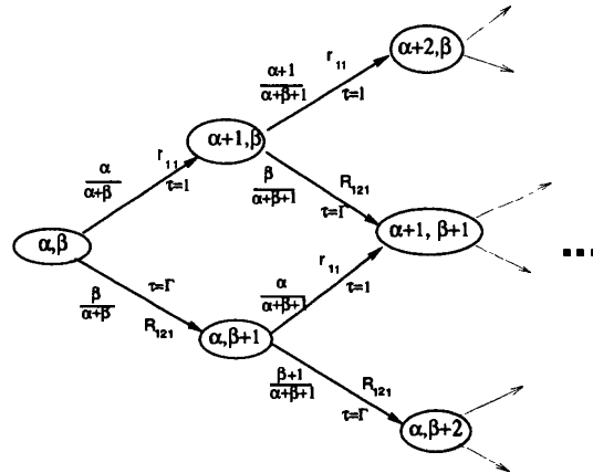
Figure 2: A local semi-Markov bandit process associated with state 1 / action 1 for the 2-state example MDP of Figure 1.
