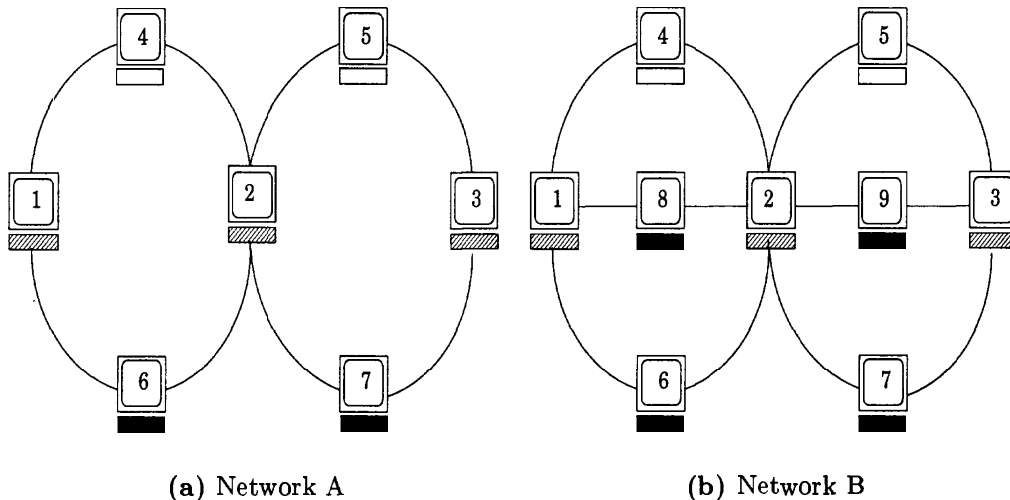
Figure 1: Network Architectures.
