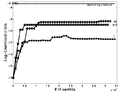
Figure 4: Learning curves for learning rates .05, .075 and .1
