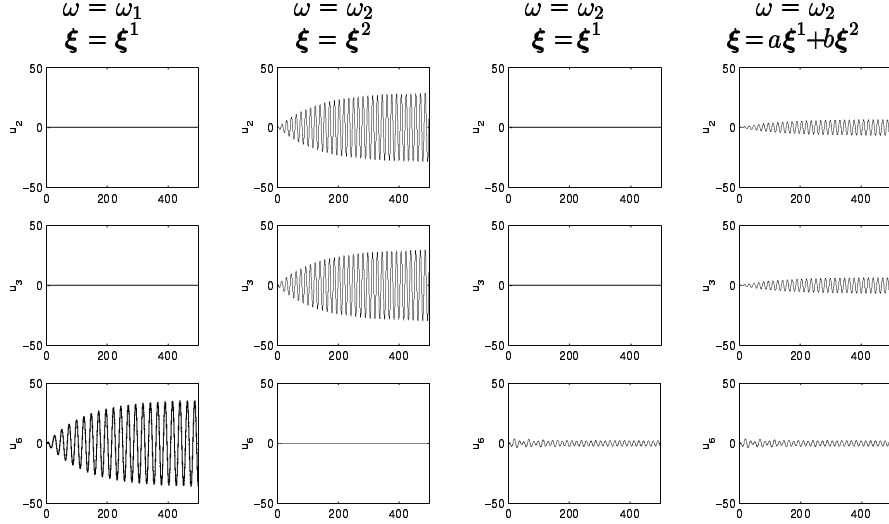
Figure 3: Frequency selectivity: Response evoked on 3 of the 10 neurons. Oscillatory patterns \xi^1 e^{-i\omega_1 t} + \text{c.c.} and \xi^2 e^{-i\omega_2 t} + \text{c.c.} have been imprinted, with \xi^1 \perp \xi^2 and \omega_1 = 41 \text{ Hz} , \omega_2 = 63 \text{ Hz} . During the learning phases the parameter a_1 of kernel was tuned appropriately, i.e. a_1 = 0.1 when imprinting \xi^1 and a_1 = 1.1 when imprinting \xi^2 .
