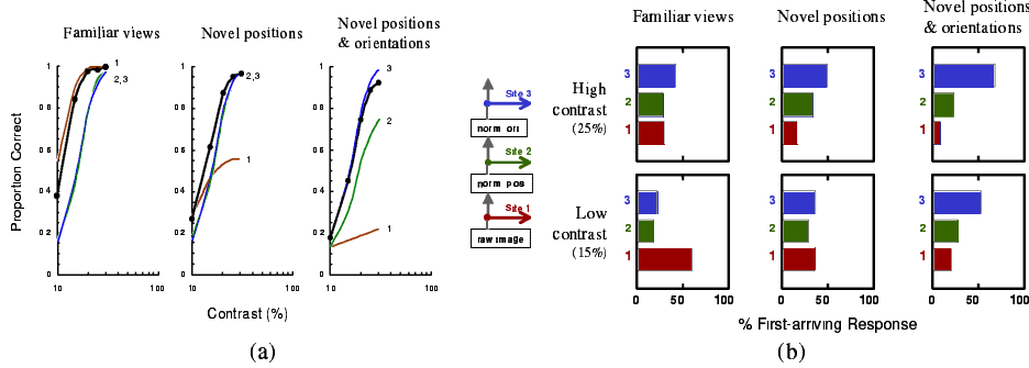
Figure 2: (a) Accuracy of the system (solid symbols) versus accuracy of each site (numbered curves) under different contrast and view conditions. (b) Relative frequency of a site issuing the first-arriving response.
