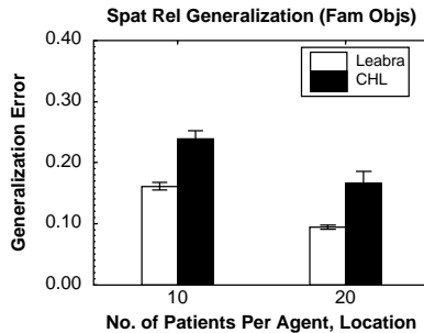
Figure 5: Generalization results for different algorithms on the spatial relationship binding task (see previous figure for details on measures) in the 400 \times 10 or 20 conditions.
