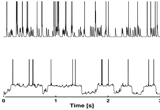
Figure 1: Inputs with high AMPA-NMDA ratio cause the cell to spike (top trace, g_{\text{AMPA}} = 0.05 , g_{\text{NMDA}} = 0.01 ). Strong NMDA inputs combined with potassium currents (for the same AMPA input) result in fluctuations of the membrane potential between two subthreshold states, with occasional firing due to the AMPA inputs (bottom trace, g_{\text{AMPA}} = 0.01 , g_{\text{NMDA}} = 0.1 )
