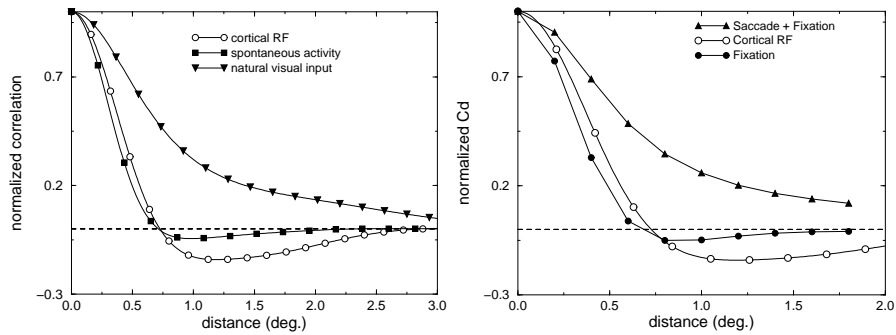
Figure 2: Analysis of the correlated activity of LGN units in different experimental conditions. In both graphs, the curve marked by white circles is the average receptive field of a simple cell, as measured by Jones and Palmer (1987) shown here for comparison. ( Left ) Static analysis: patterns of correlated activity in the presence of spontaneous activity and when natural visual input was analyzed statically. ( Right ) Effects of eye movements: correlation difference functions measured when natural images were scanned with sequence or saccades or fixational eye movements.
