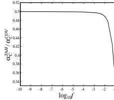
Figure 5 !! The comparison of the storage capacity of our model with that of the model using the covariance learning. As f decreases, the ratio of storage capacity approaches 0.5.
