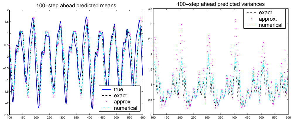
Figure 2: 100-step ahead mean predictions (left) and uncertainties (right) obtained using the exact method (dash), the approximate (dot) and the sample mean and variance of the numerical solution (dash-dot).
