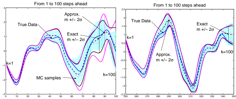
Figure 1: Iterative method in action: simulation from 1 to 100 steps ahead for different starting points in the test series. Mean predictions with 2\sigma error bars given by the exact (dash) and approximate (dot) methods. Also plotted, 50 samples obtained using the numerical approximation.
