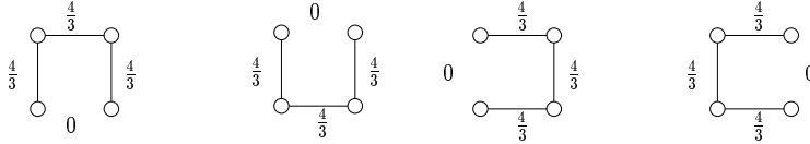
Figure 1. A convex combination of four distributions p(\mathbf{x}; \theta(\mathcal{T}_i)) , each defined by a spanning tree \mathcal{T}_i , is used to approximate the target distribution p(\mathbf{x}; \hat{\theta}) on the single-cycle graph.
