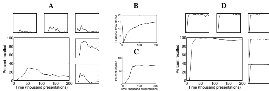
Figure 2: How semantic training affects episodic recall for patterns stored after the first 10,000 presentations ( A ) without replay and ( D ) with the correspondence between hippocampal and neocortical representations updated during off-line replay. The larger graphs are averages over all stored episodes, while the smaller graphs are for individual episodes. Recall was assessed by presenting partial episodic patterns (the original activations replaced by random patterns in one of the input areas), performing hippocampal pattern completion in EP if the distance from a stored EP representation was less than 20, and then performing 20 full iterations of Gibbs sampling in the neocortical network with the cue areas clamped. A resulting distance of less than 5 from the target pattern was considered a match. ( B ) and ( C ) analyze the reasons why episodic recall breaks down in ( A ). ( B ) shows how the EP representation of stored episodes drifts away from the original stored patterns. ( C ) shows how well recall works if it starts from the stored EP representation of the episode.
