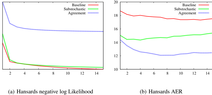
Figure 4: Data likelihood and AER vs. EM iteration using HMM on 100k Hansards.
