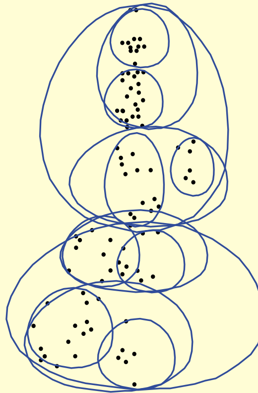
Space decomposition
