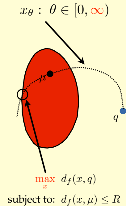
Geometry
