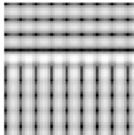
MODEL SALIENCY
