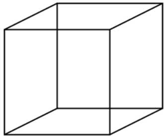
Necker cube
