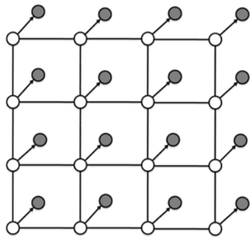
Markov random field image models
