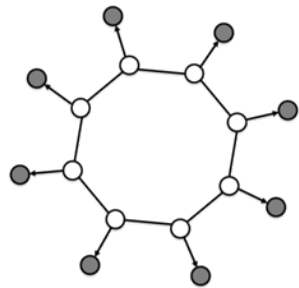
Markov random field image models
